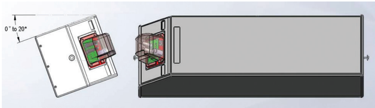
Figure 1 Orientation of the rain hood and tilt angle limitation of the USW-210P speaker with rain hood option.
