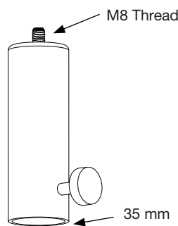
PAS-M8 Adapter Sleeve M8 (35 MM Pole) (PN 40.010.975.01)
