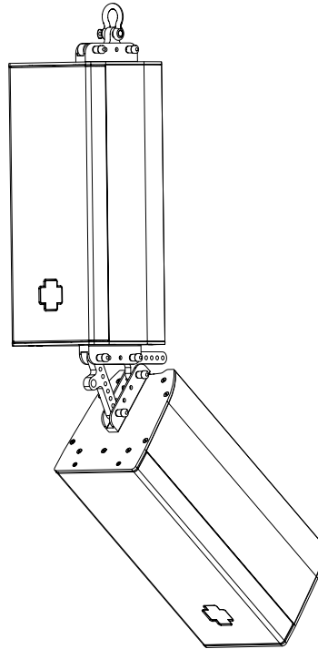
Two MTC-X20 Top Channels linking speakers (a third MTC-X20 on top).
